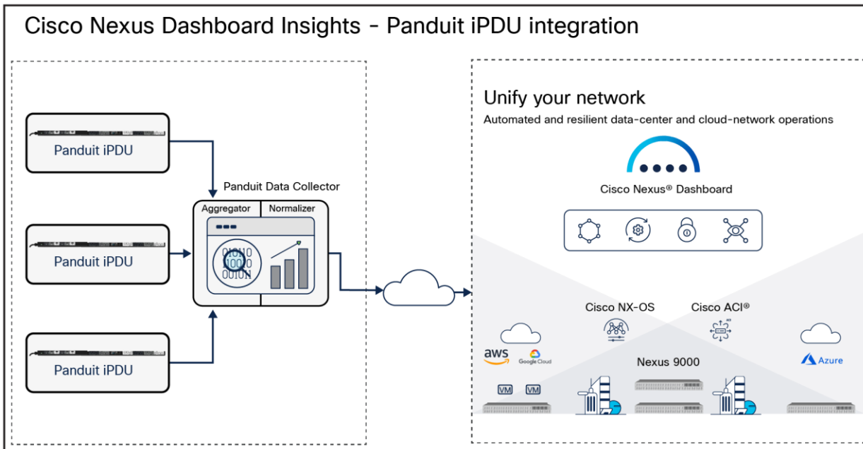
Figure 2. Solution architecture
